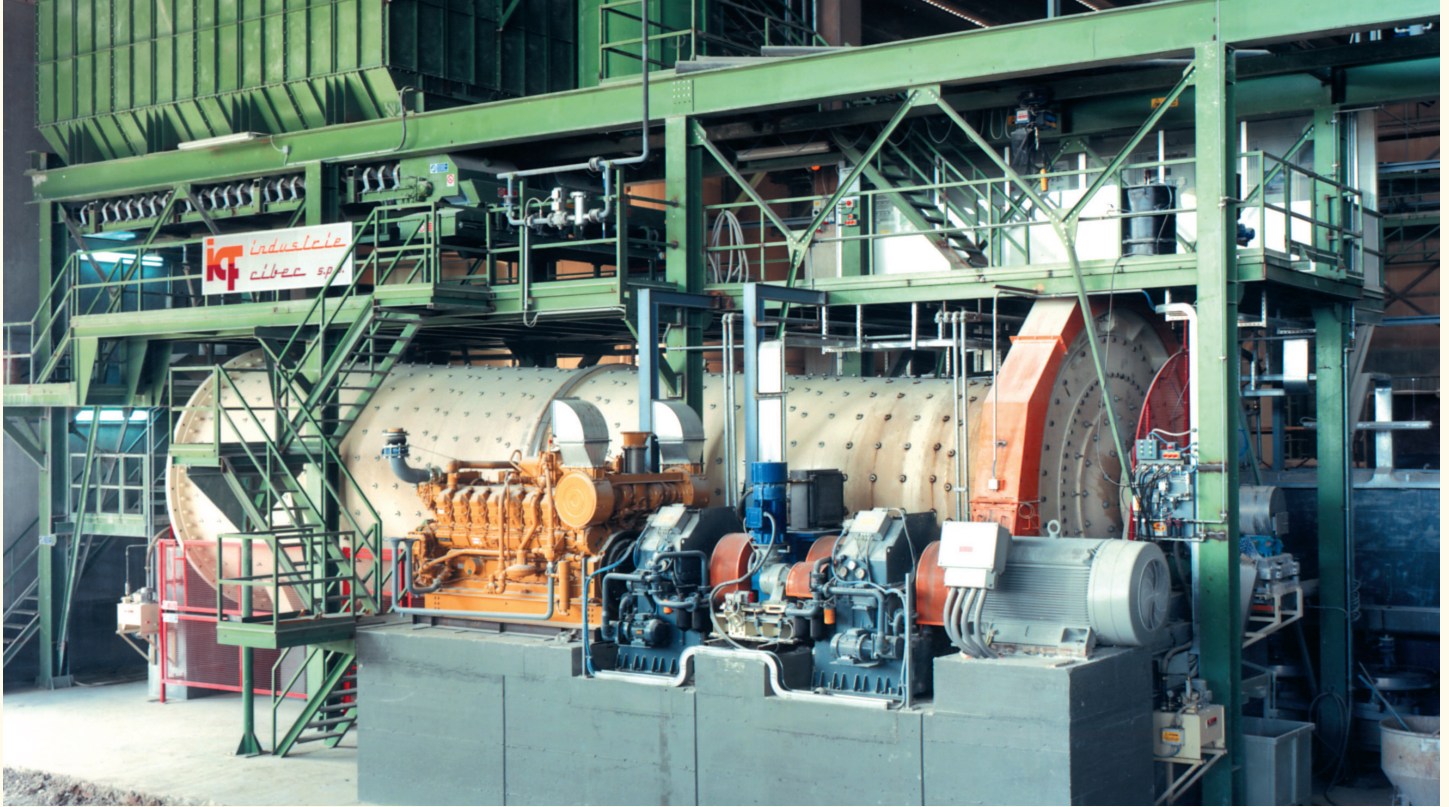
2x34 KSL, 630 kW - 1000 rpm, Ceramic mill (Italy)
